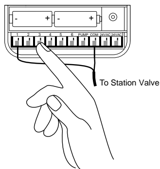
FIGURE 24: Connecting Valve Wires
