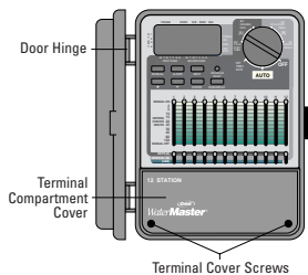
FIGURE 21: Outdoor Timer, Showing Terminal Cover
